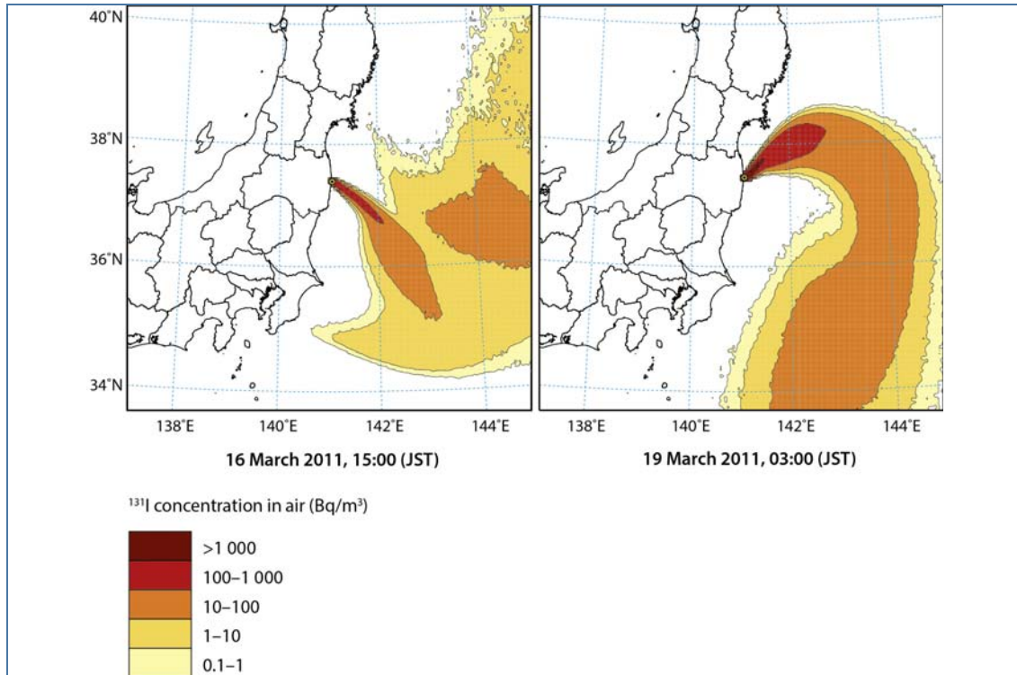
Figure B-XI. Simulated air concentration of ^{131}\text{I} during subsequent releases from FDNPS
